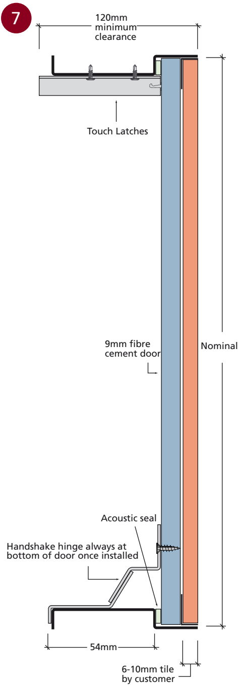
7 ■ INSTALLATION DETAIL
